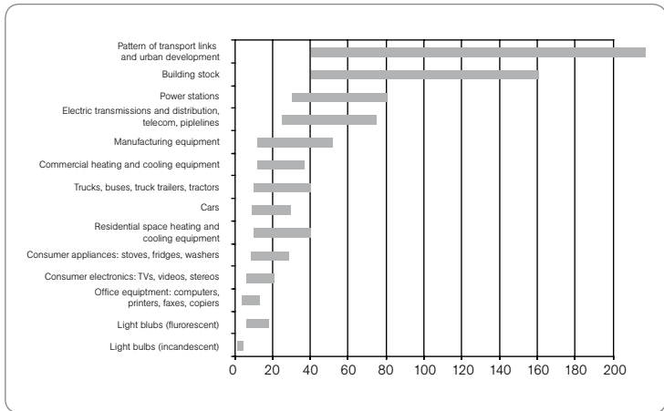
Figure 20: Average lifespans for selected energy/related capital stock 348
