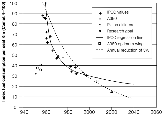
Figure 21. Long-haul aircraft efficiency gains since 1950 as an index based on the De Havilland H106 Comet 4.
