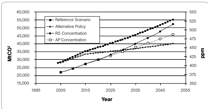
Figure 6. IEA scenario emissions and resulting atmospheric CO 2 concentrations.
